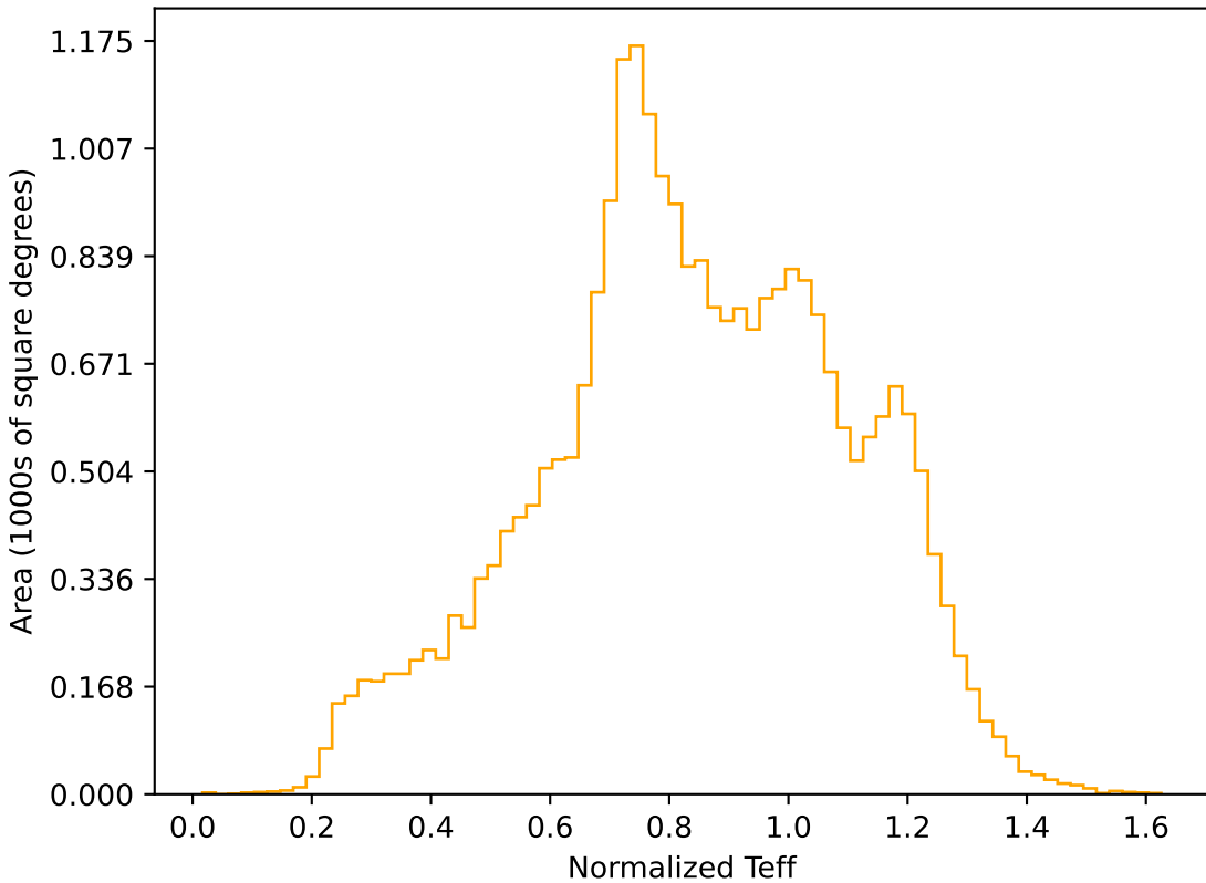
noroll_mjdp270_v3.4_10yrs All sky r band: Normalized Teff
