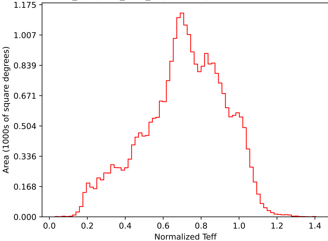
noroll_mjdp270_v3.4_10yrs All sky i band: Normalized Teff
