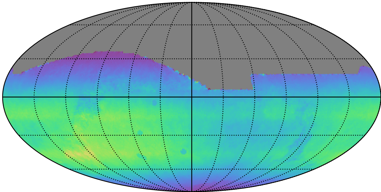
noroll_mjdp270_v3.4_10yrs All sky all bands: Normalized Teff
