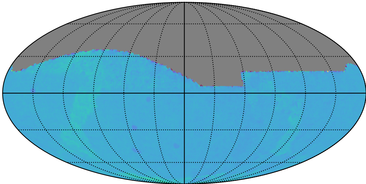
noroll_mjdp270_v3.4_10yrs All sky: Normalized Proper Motion Uncert @ 20.5
