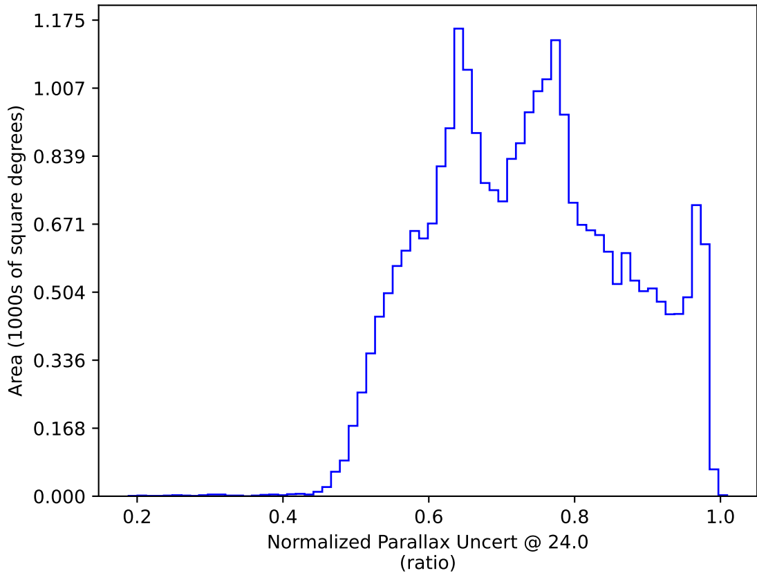
noroll_mjdp270_v3.4_10yrs All sky: Normalized Parallax Uncert @ 24.0
