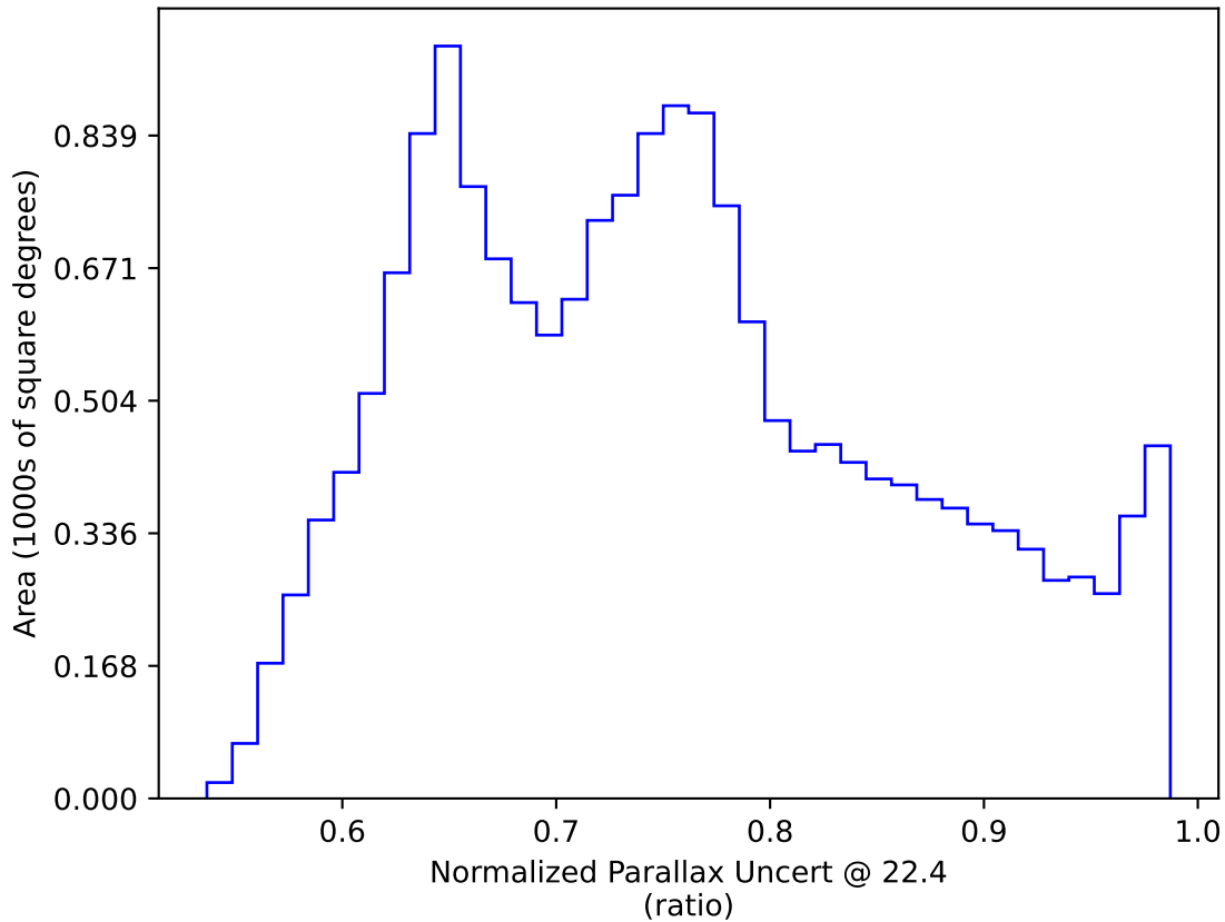
noroll_mjdp270_v3.4_10yrs WFD: Normalized Parallax Uncert @ 22.4
