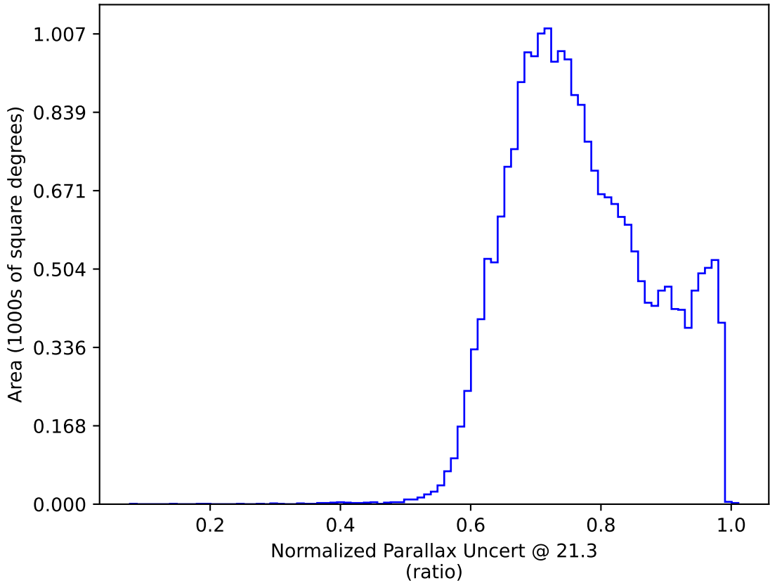
noroll_mjdp270_v3.4_10yrs All sky y band only: Normalized Parallax Uncert @ 21.3
