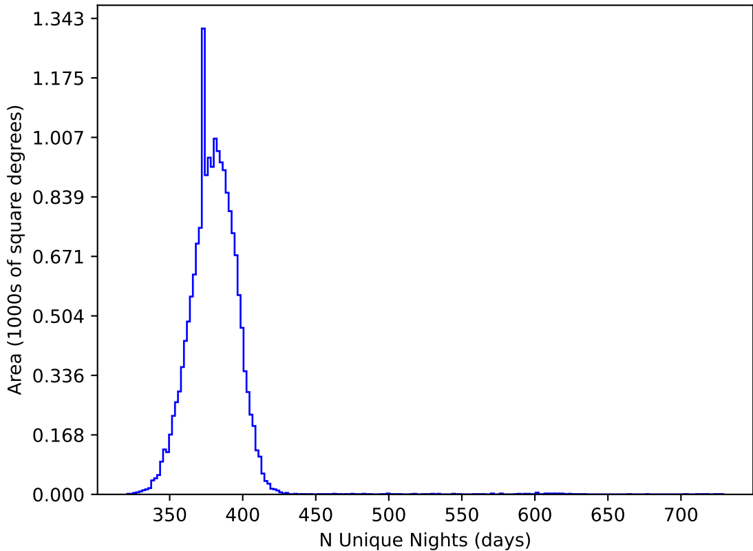
noroll_mjdp270_v3.4_10yrs WFD all bands: N Unique Nights
