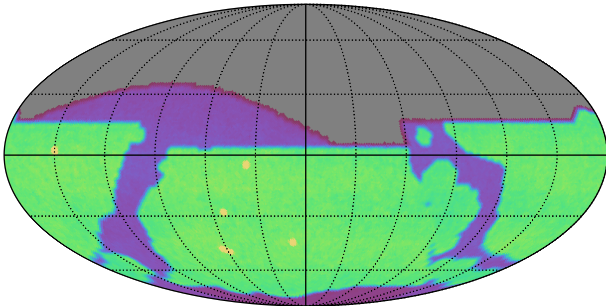
noroll_mjdp270_v3.4_10yrs All sky all bands: N Unique Nights
