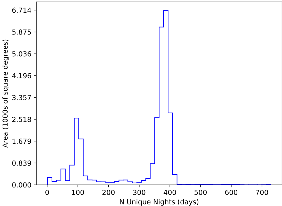
noroll_mjdp270_v3.4_10yrs All sky all bands: N Unique Nights
