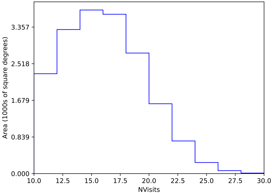
noroll_mjdp270_v3.4_10yrs Yr 3-4 y band: NVisits
