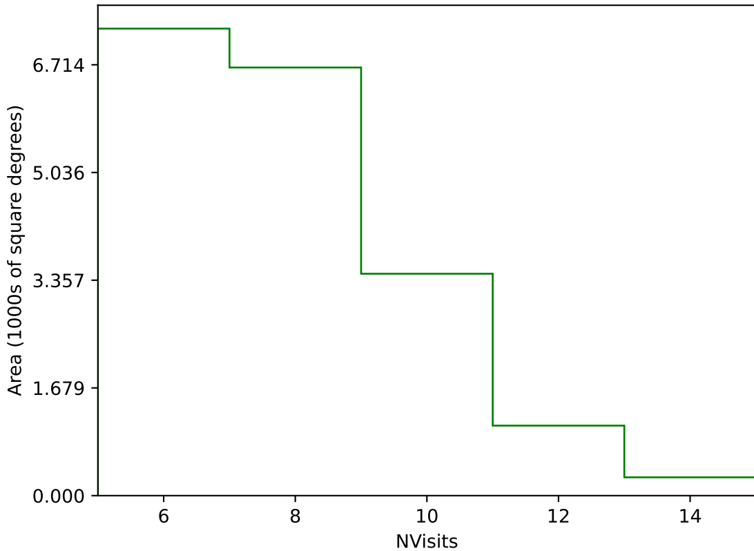
noroll_mjdp270_v3.4_10yrs Yr 3-4 g band: NVisits
