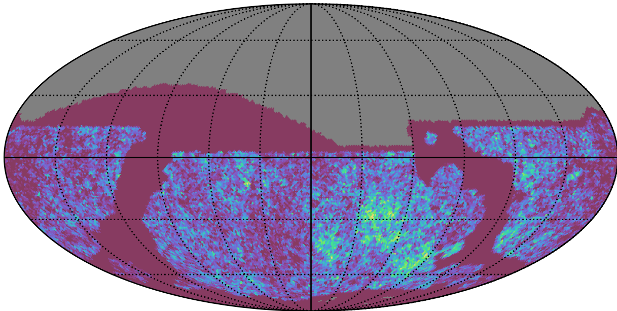
noroll_mjdp270_v3.4_10yrs Yr 3-4 all bands: NVisits
