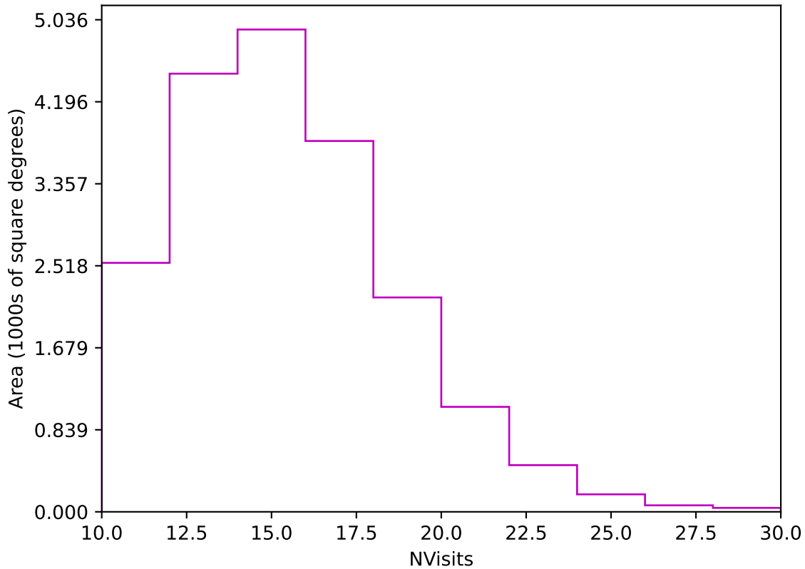
noroll_mjdp270_v3.4_10yrs Yr 1 z band: NVisits
