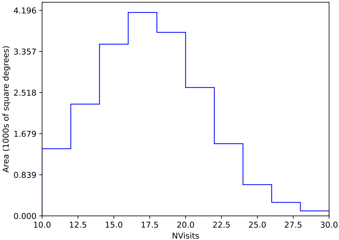
noroll_mjdp270_v3.4_10yrs Yr 1 y band: NVisits
