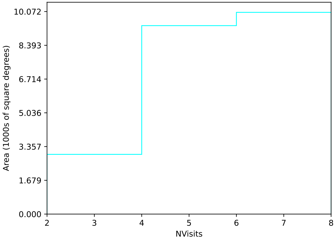
noroll_mjdp270_v3.4_10yrs Yr 1 u band: NVisits
