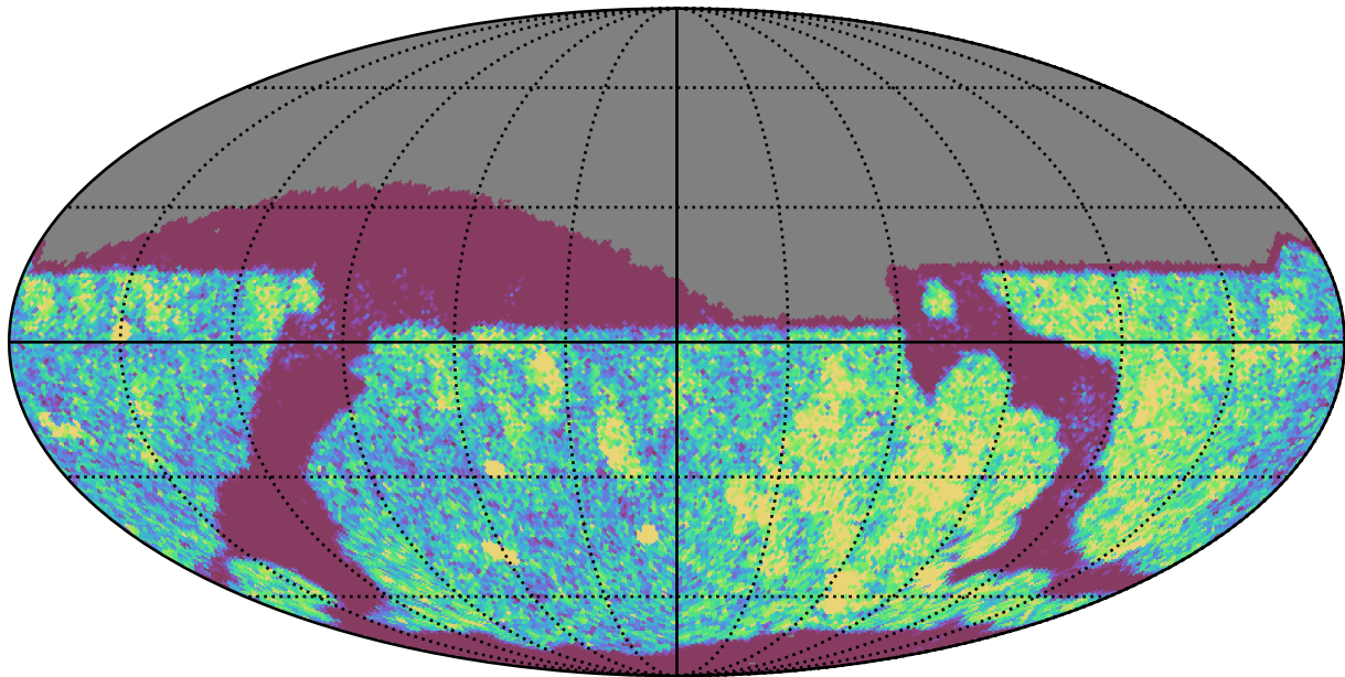
noroll_mjdp270_v3.4_10yrs Yr 1 i band: NVisits
