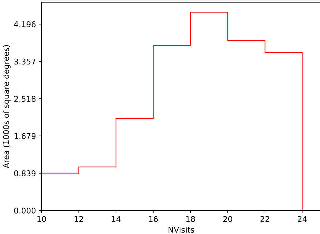
noroll_mjdp270_v3.4_10yrs Yr 1 i band: NVisits
