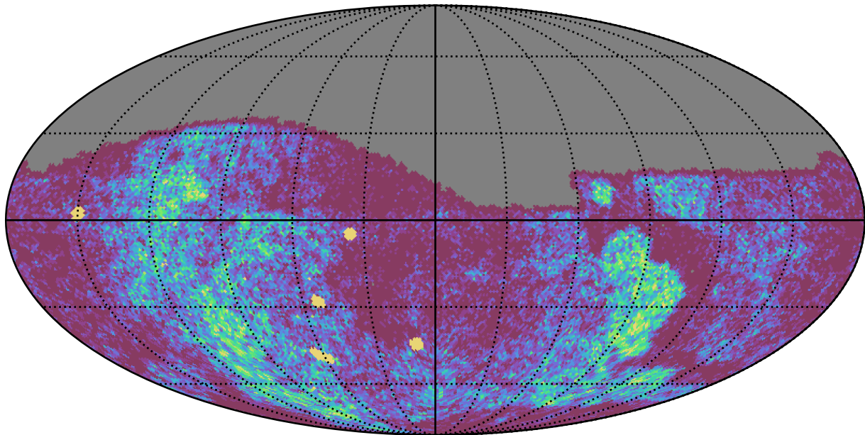
noroll_mjdp270_v3.4_10yrs Yr 1 g band: NVisits
