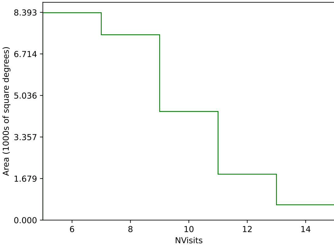
noroll_mjdp270_v3.4_10yrs Yr 1 g band: NVisits
