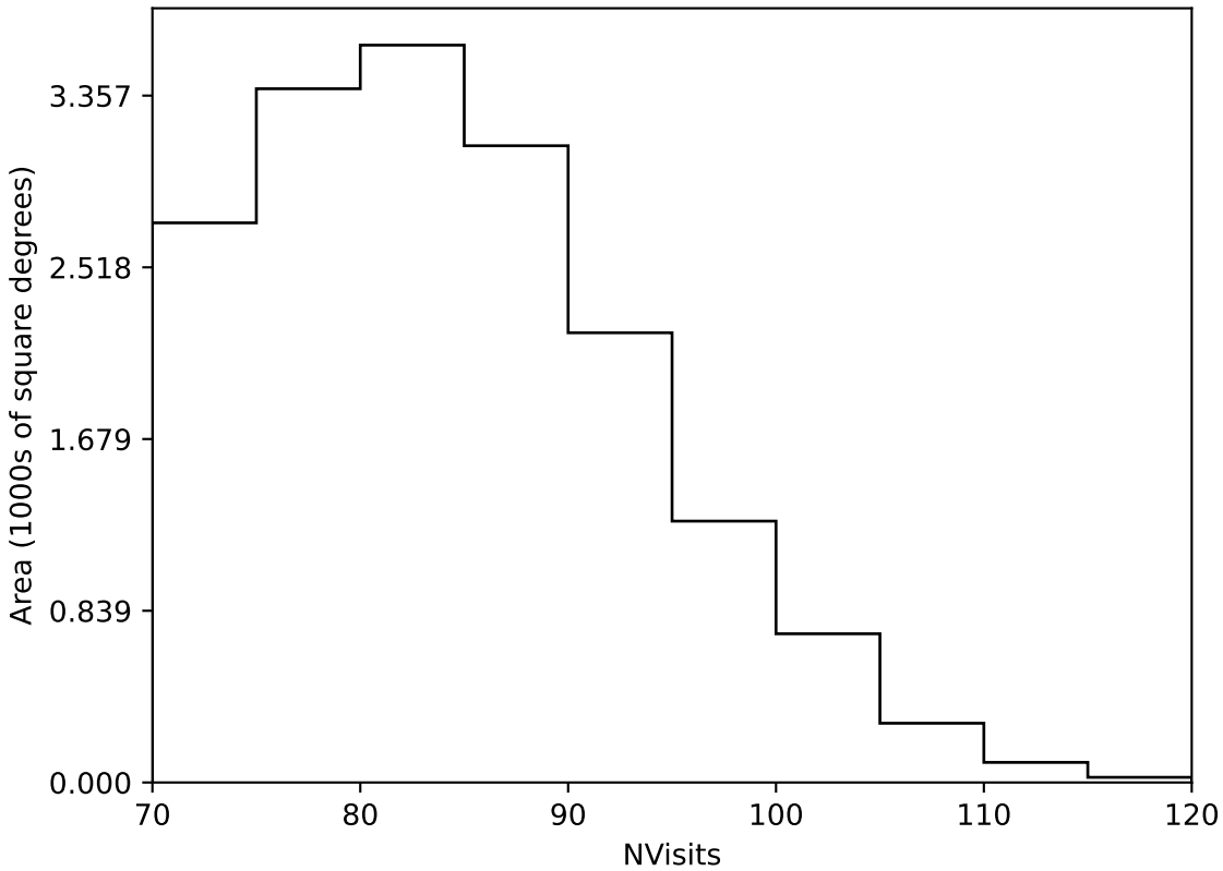
noroll_mjdp270_v3.4_10yrs Yr 1 all bands: NVisits
