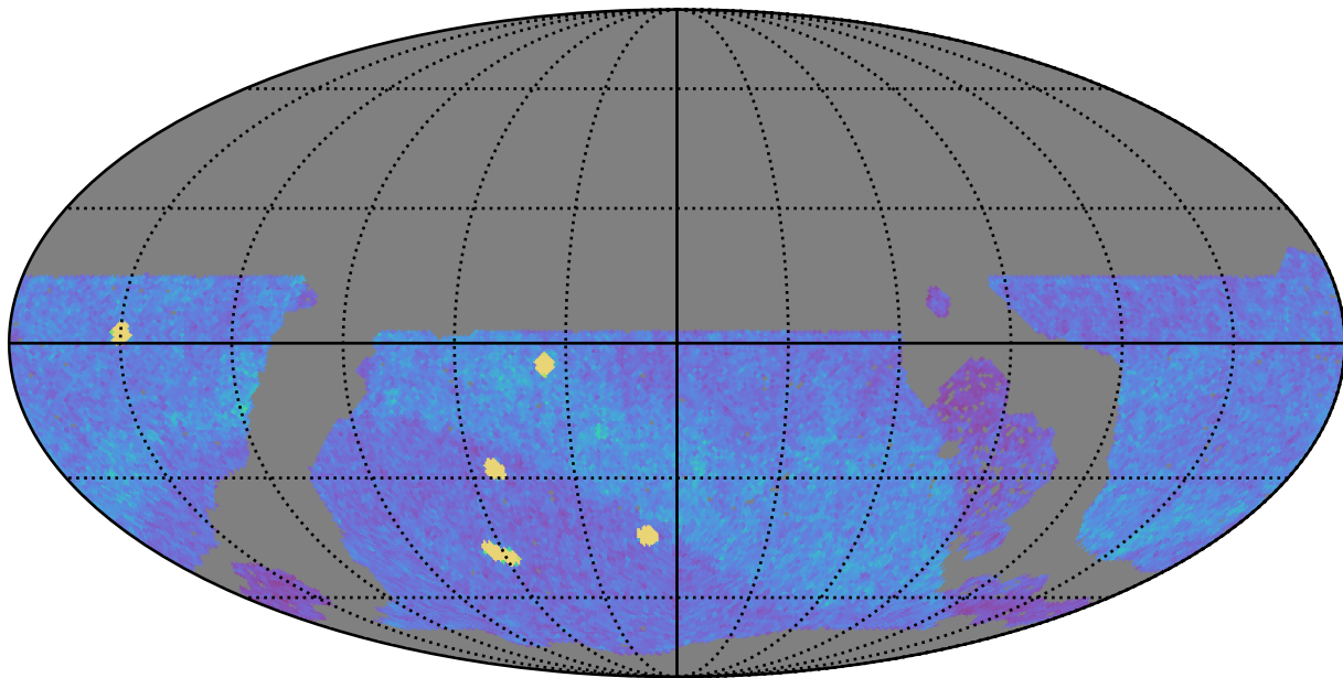
noroll_mjdp270_v3.4_10yrs WFD z band: NVisits
