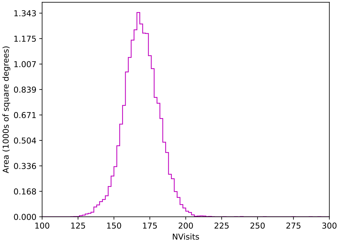
noroll_mjdp270_v3.4_10yrs WFD z band: NVisits
