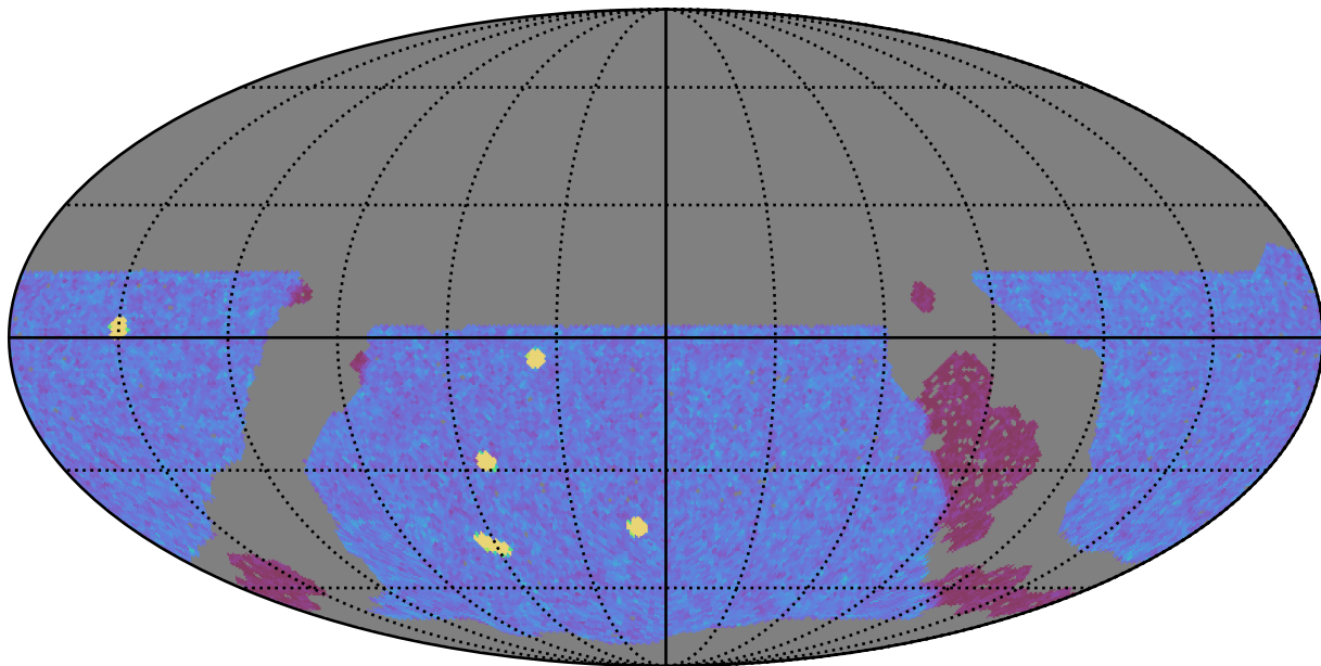
noroll_mjdp270_v3.4_10yrs WFD y band: NVisits
