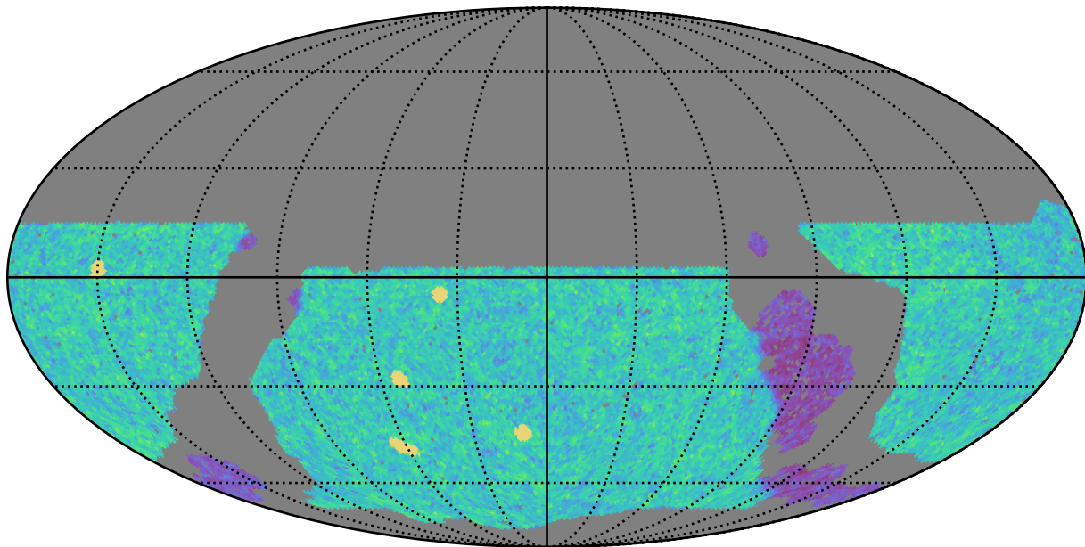
noroll_mjdp270_v3.4_10yrs WFD u band: NVisits
