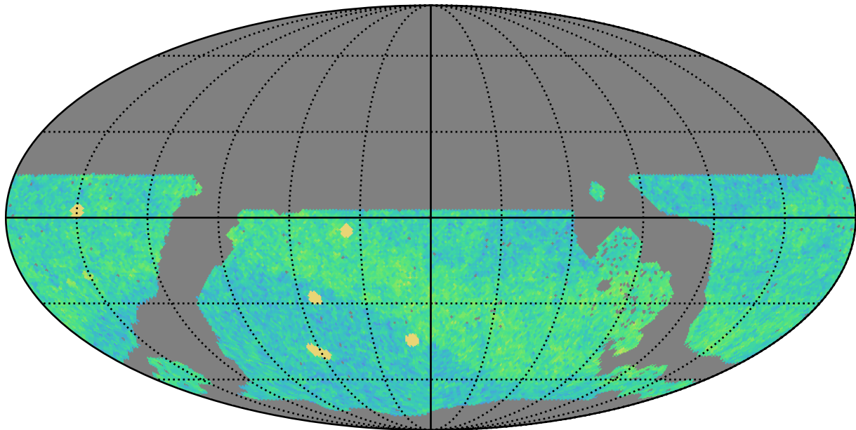
noroll_mjdp270_v3.4_10yrs WFD i band: NVisits
