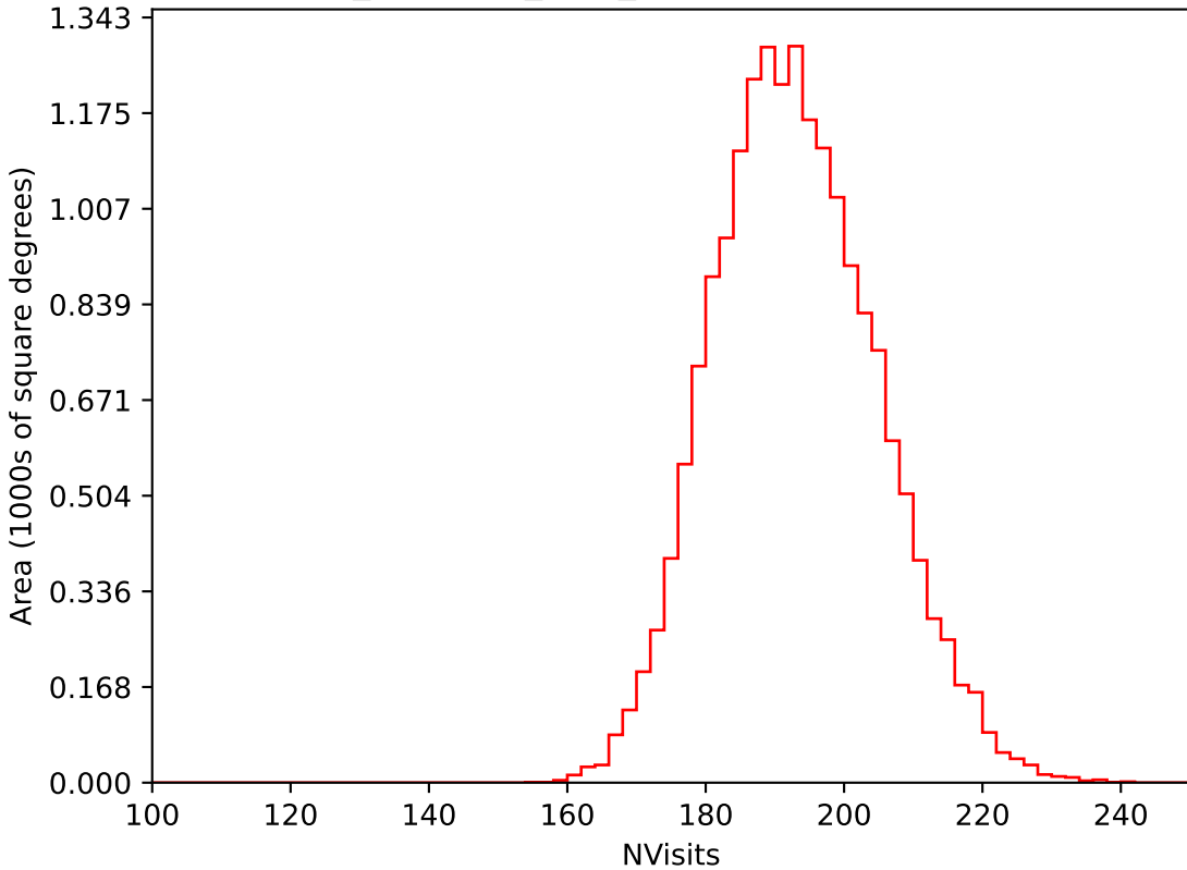
noroll_mjdp270_v3.4_10yrs WFD i band: NVisits
