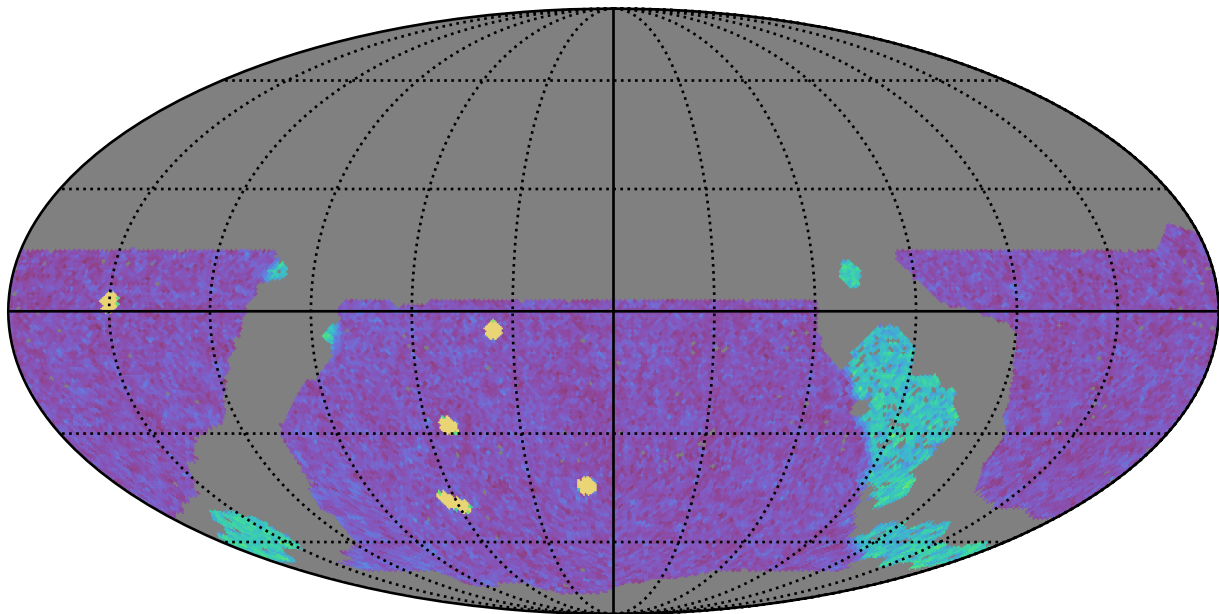
noroll_mjdp270_v3.4_10yrs WFD g band: NVisits
