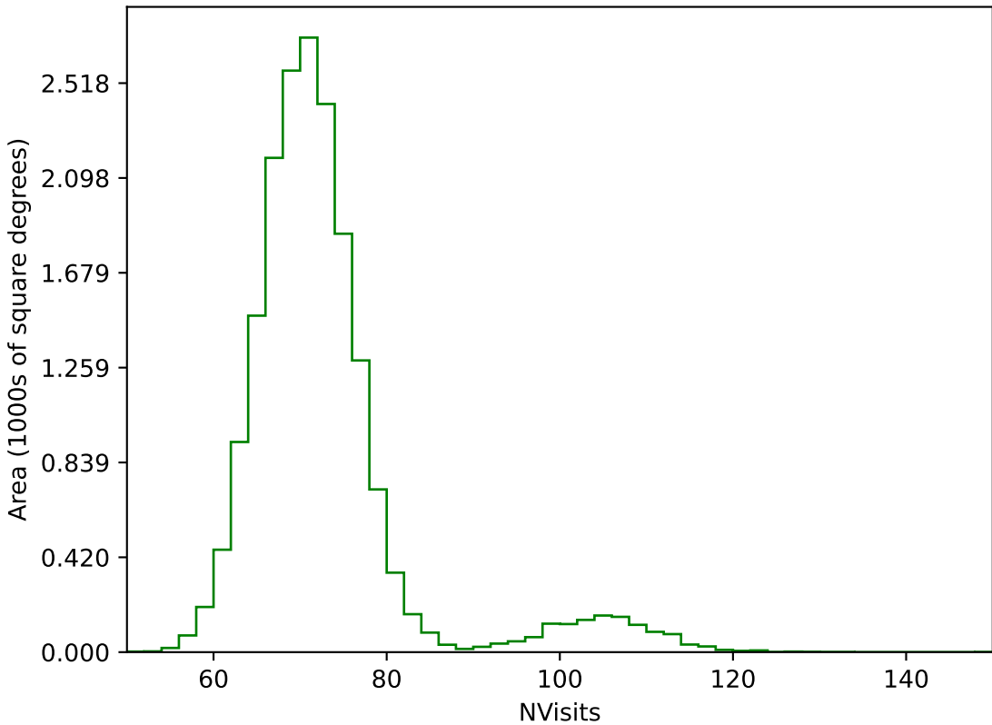
noroll_mjdp270_v3.4_10yrs WFD g band: NVisits
