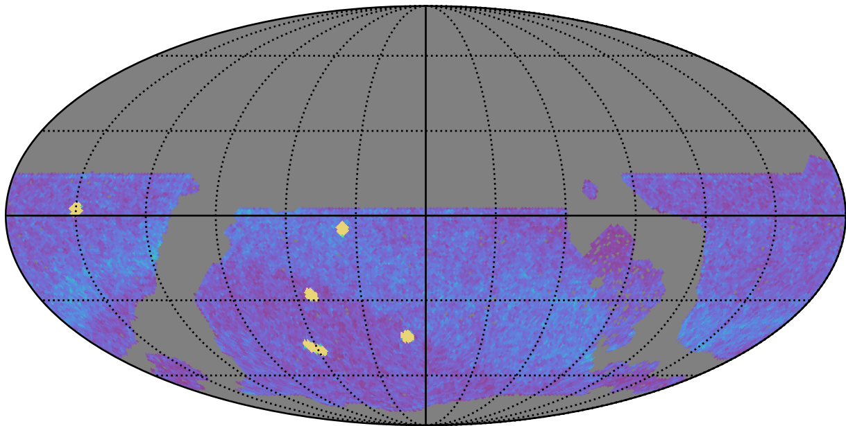
noroll_mjdp270_v3.4_10yrs WFD all bands: NVisits
