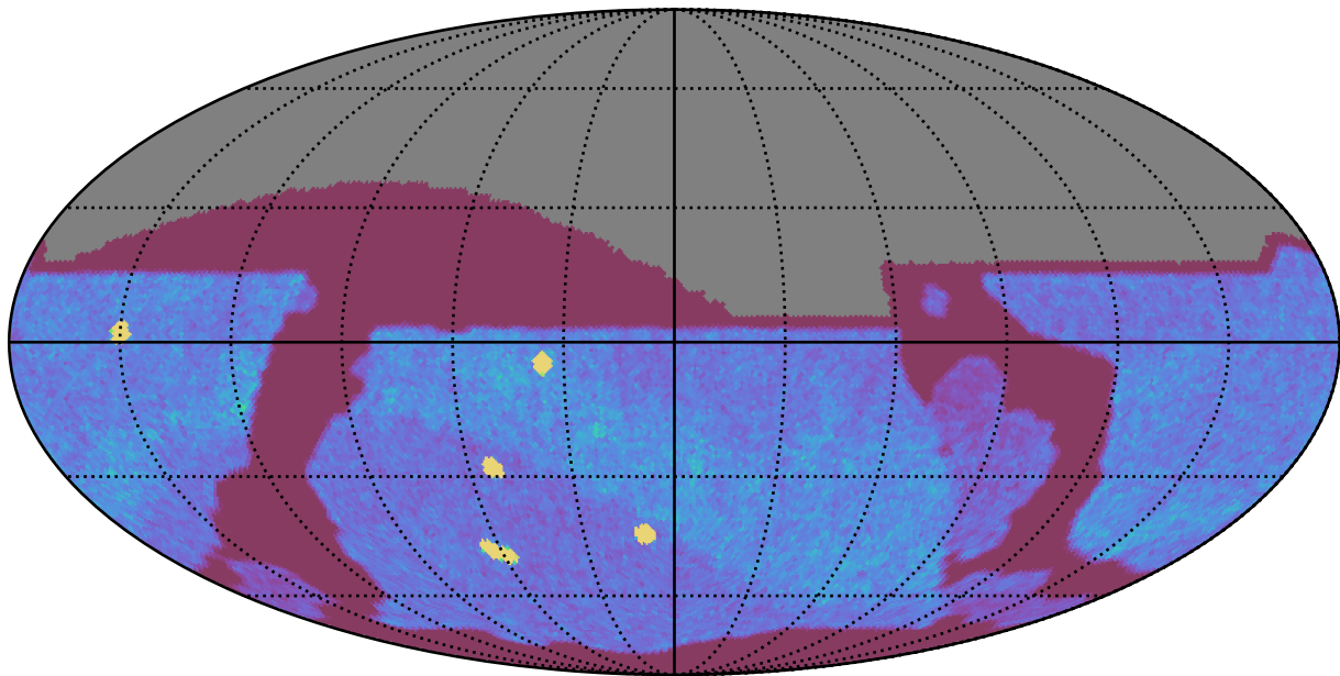
noroll_mjdp270_v3.4_10yrs All sky z band: NVisits
