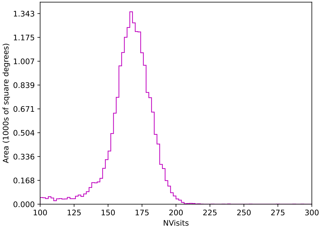
noroll_mjdp270_v3.4_10yrs All sky z band: NVisits
