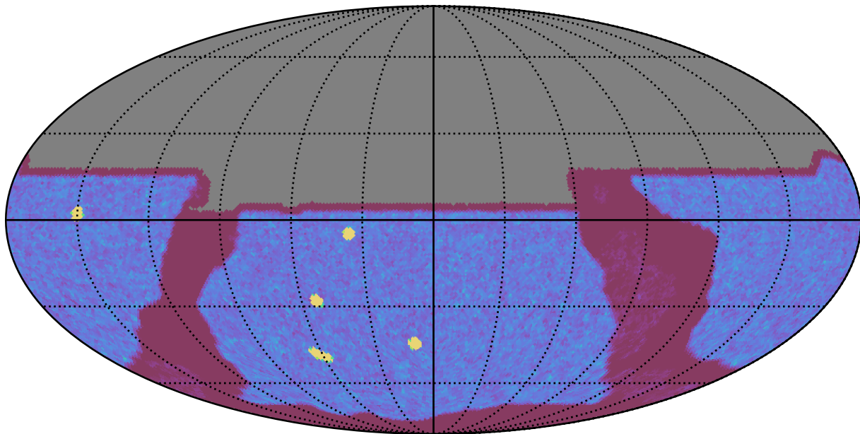
noroll_mjdp270_v3.4_10yrs All sky y band: NVisits
