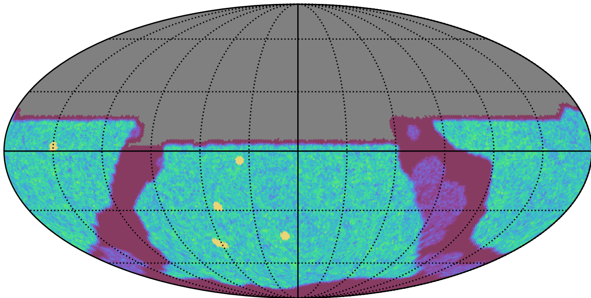
noroll_mjdp270_v3.4_10yrs All sky u band: NVisits
