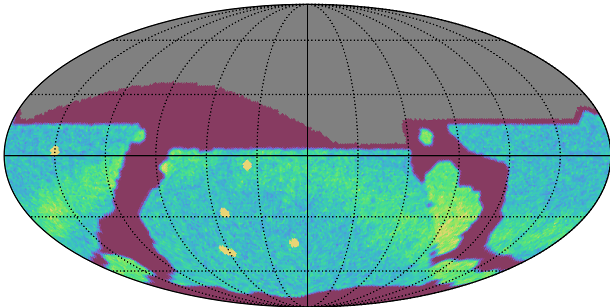
noroll_mjdp270_v3.4_10yrs All sky r band: NVisits
