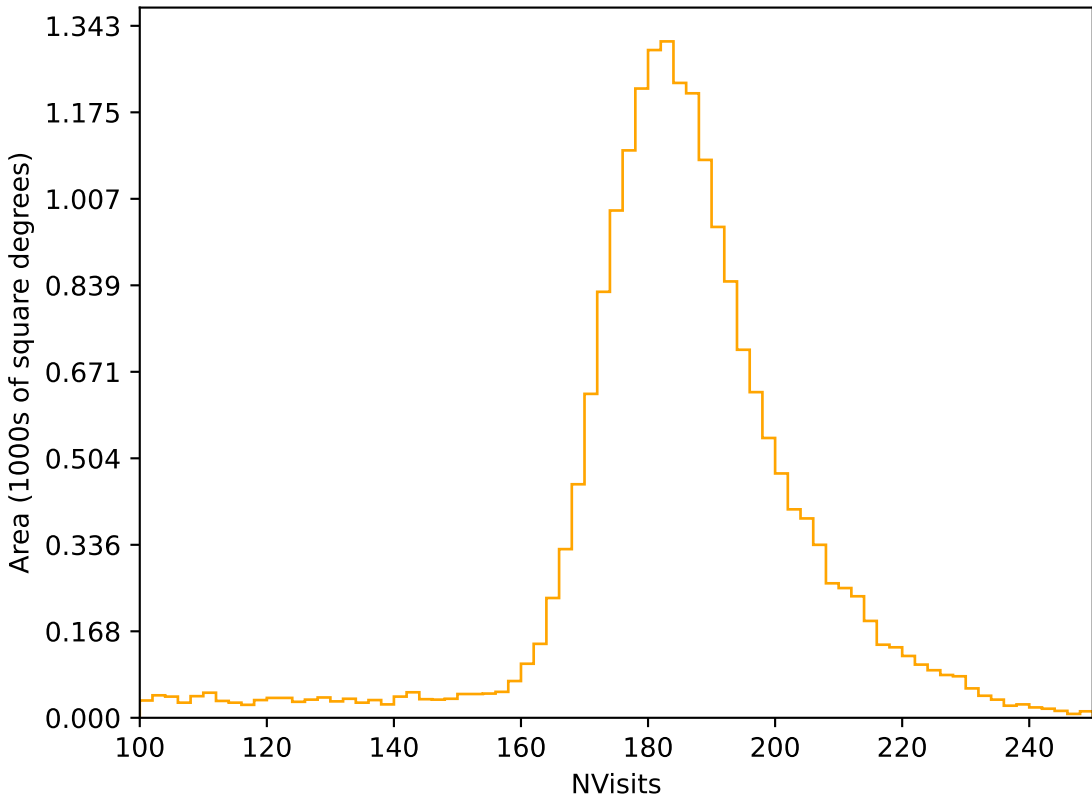
noroll_mjdp270_v3.4_10yrs All sky r band: NVisits
