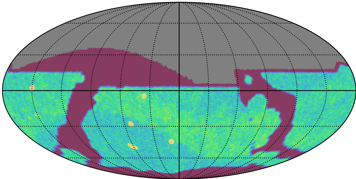
noroll_mjdp270_v3.4_10yrs All sky i band: NVisits
