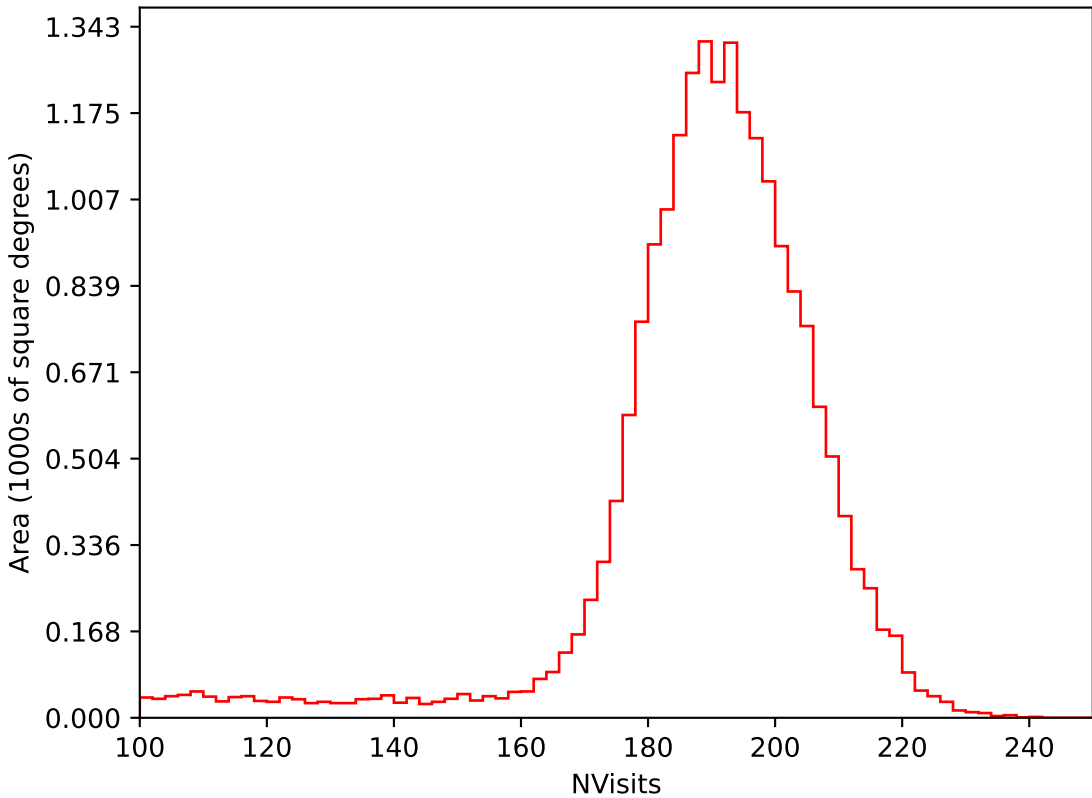
noroll_mjdp270_v3.4_10yrs All sky i band: NVisits
