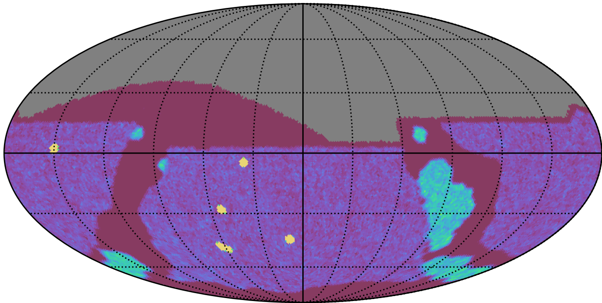
noroll_mjdp270_v3.4_10yrs All sky g band: NVisits
