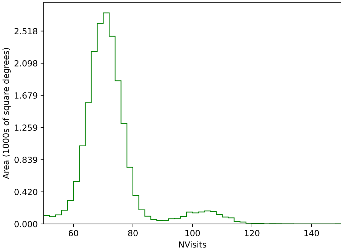
noroll_mjdp270_v3.4_10yrs All sky g band: NVisits
