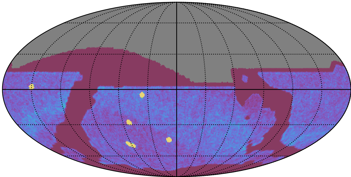
noroll_mjdp270_v3.4_10yrs All sky all bands: NVisits
