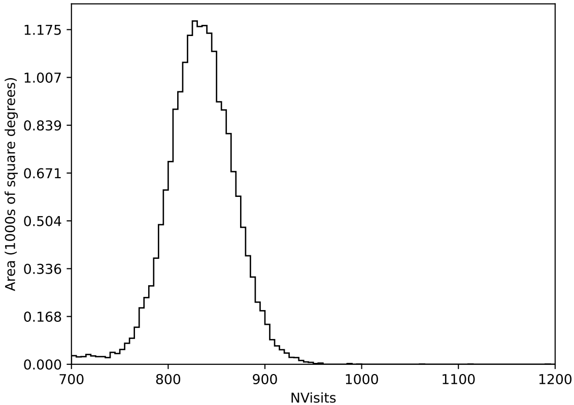
noroll_mjdp270_v3.4_10yrs All sky all bands: NVisits
