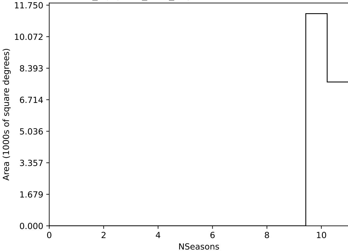
noroll_mjdp270_v3.4_10yrs WFD all bands: NSeasons
