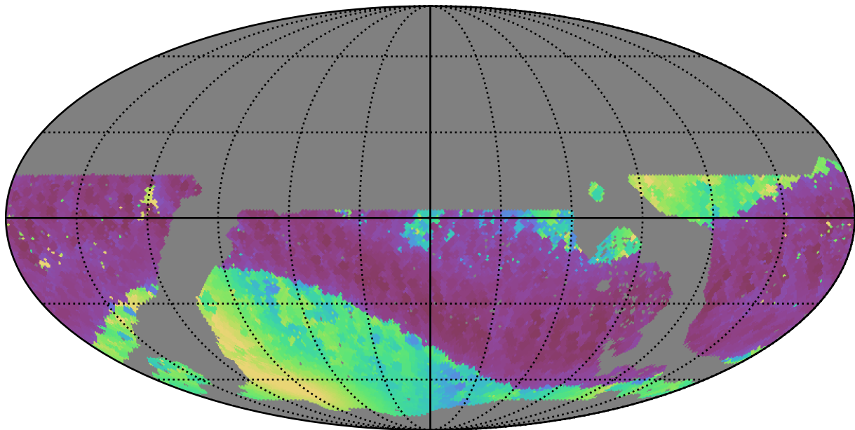
noroll_mjdp270_v3.4_10yrs WFD z band: Min solarElong
