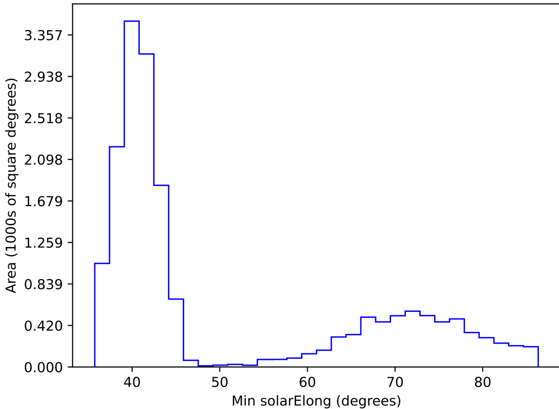
noroll_mjdp270_v3.4_10yrs WFD z band: Min solarElong
