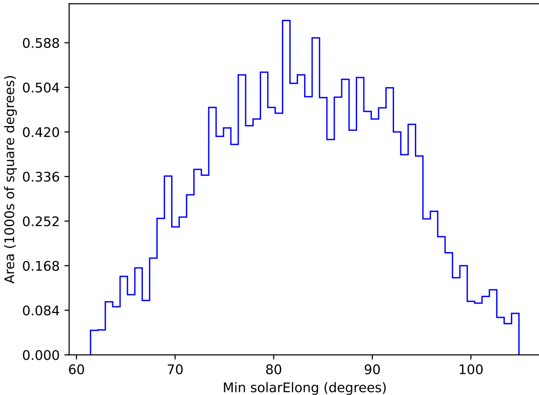
noroll_mjdp270_v3.4_10yrs WFD u band: Min solarElong
