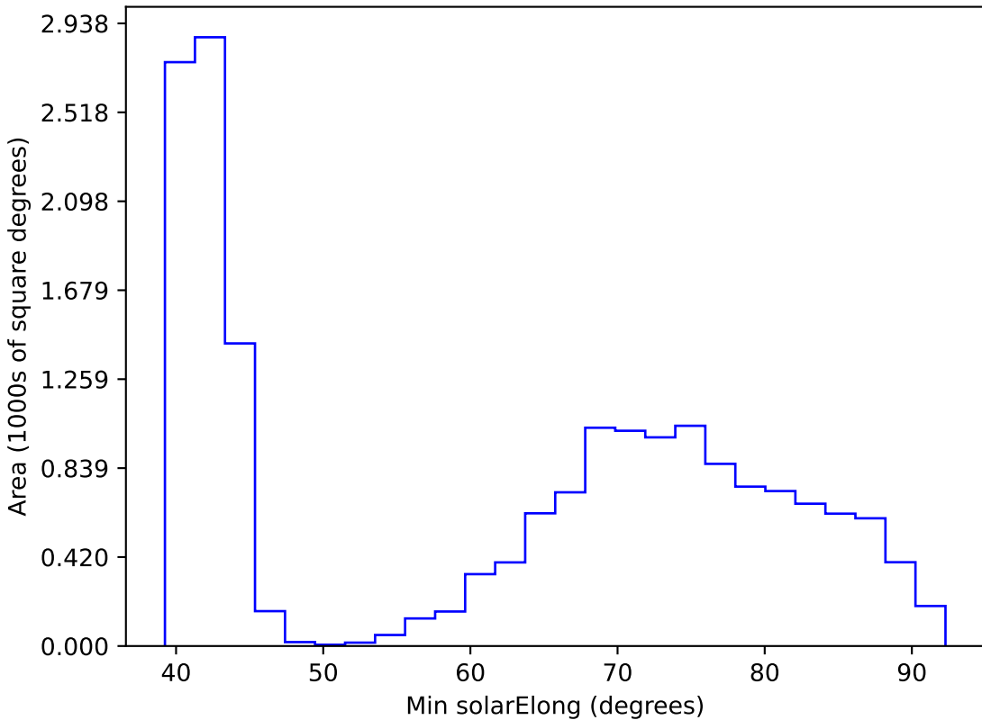
noroll_mjdp270_v3.4_10yrs WFD r band: Min solarElong
