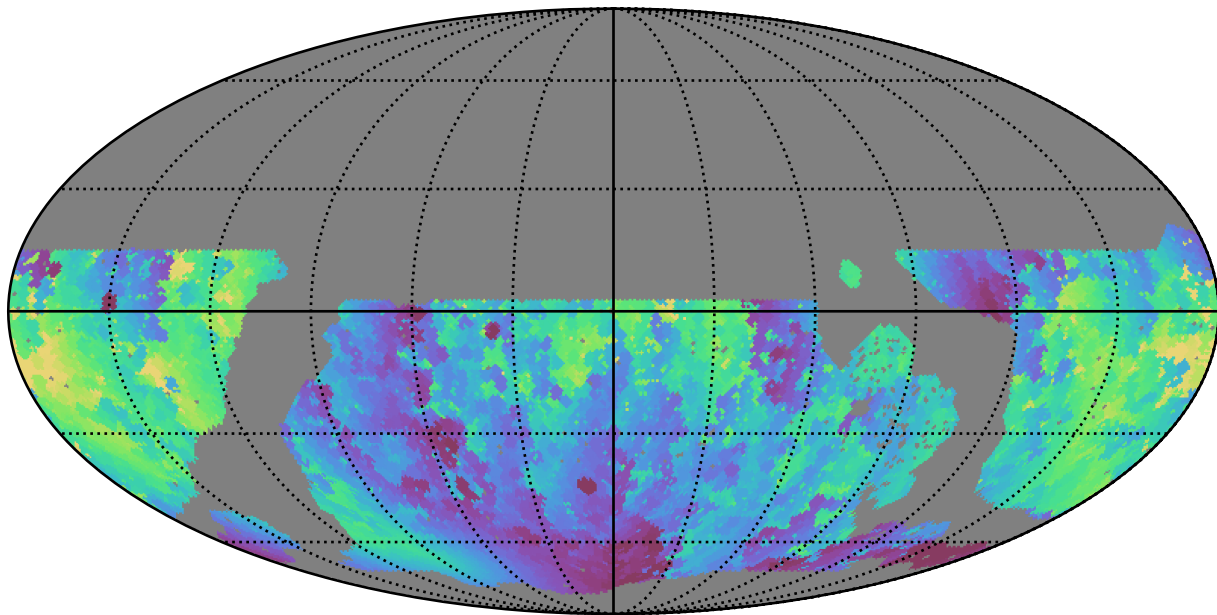
noroll_mjdp270_v3.4_10yrs WFD g band: Min solarElong
