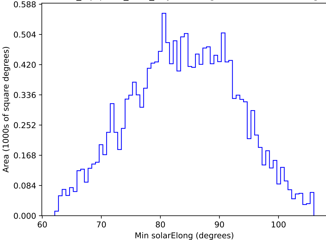
noroll_mjdp270_v3.4_10yrs WFD g band: Min solarElong
