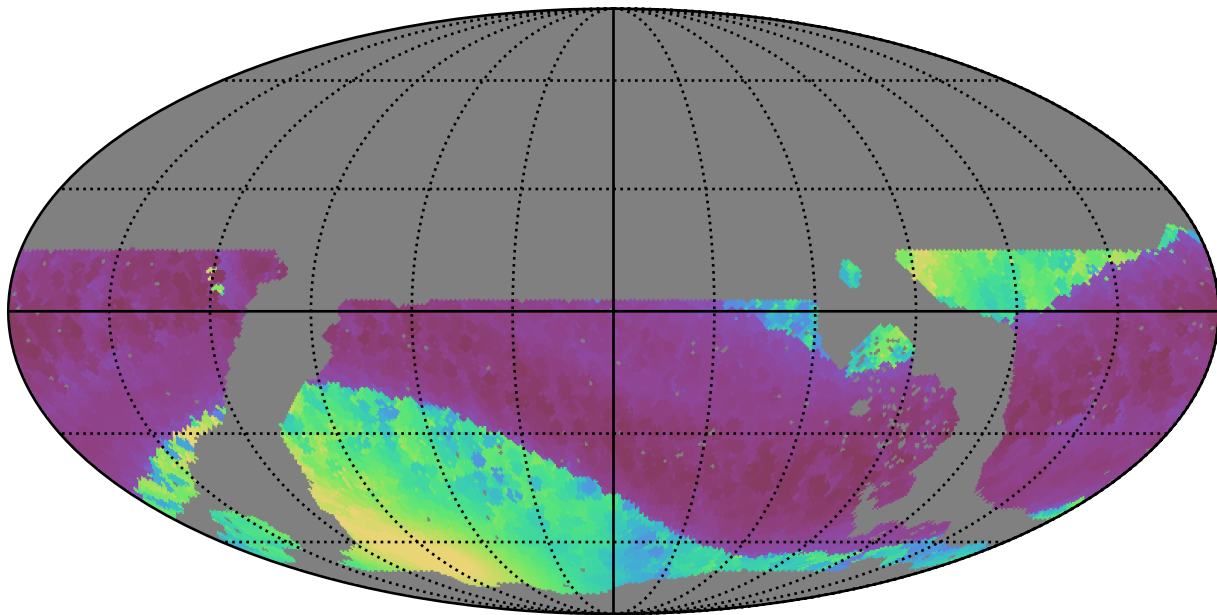
noroll_mjdp270_v3.4_10yrs WFD all bands: Min solarElong
